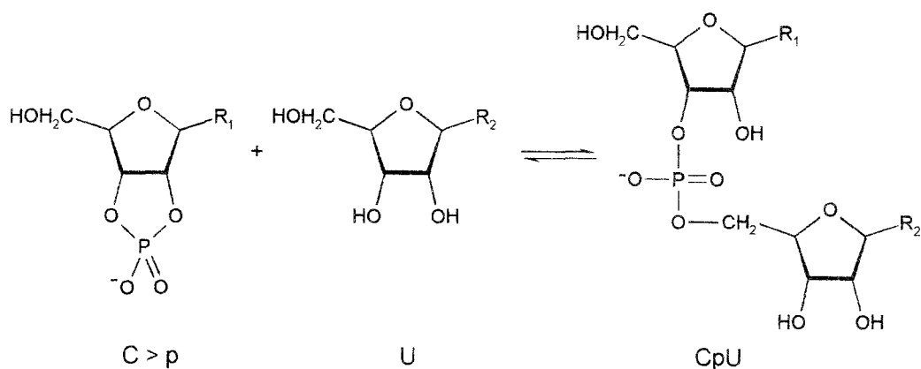
Scheme 4. Ribonuclease A-catalysed synthesis of cytidyl(3'-5')uridine from cytidine 2':3'-cyclic monophosphate and uridine. \text{C} > \text{p} , cytidine 2':3'-cyclic monophosphate, \text{U} , uridine, \text{CpU} , cytidyl(3'-5')uridine; R_1 , cytosine, R_2 , uracile
